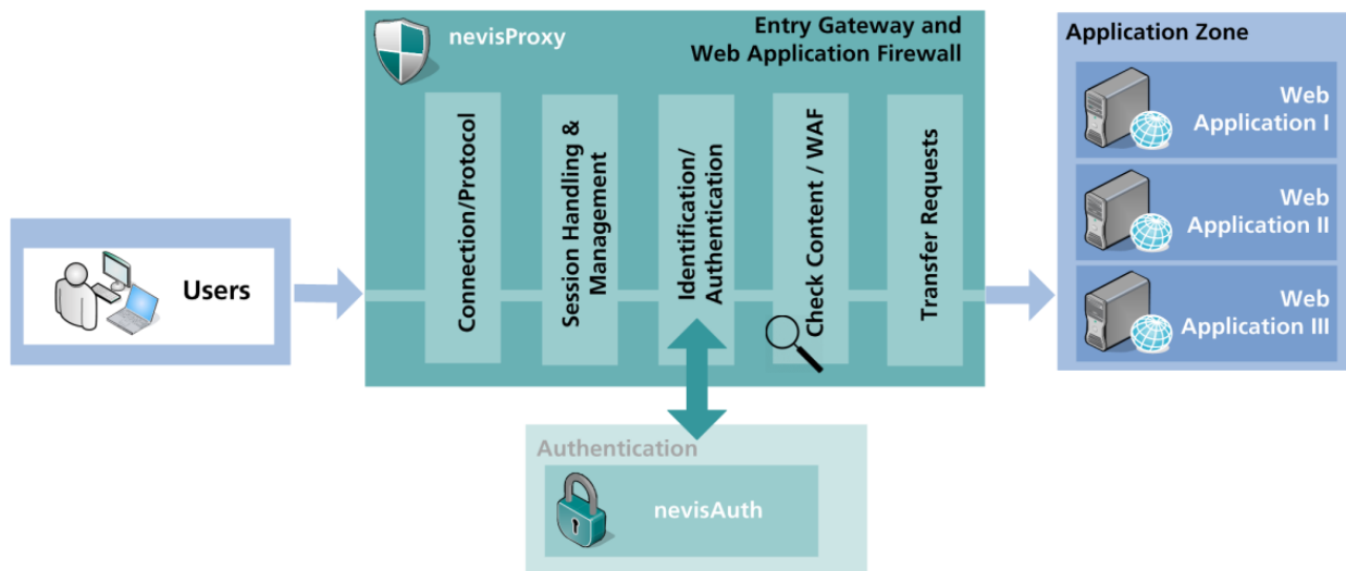
Figure 1 nevisProxy - overview
